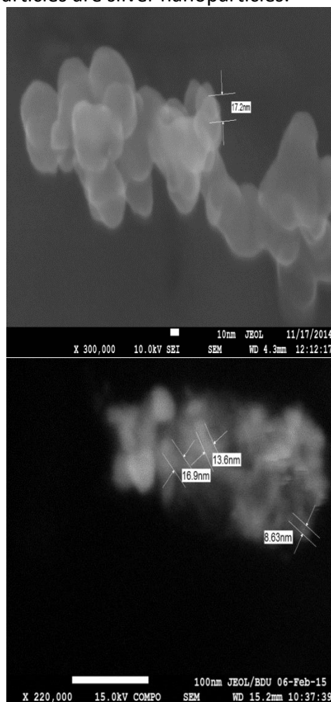
Fig.3. Scanning electron microscopy of silver nanoparticles synthesized by Saccharomyces sp. BDU-XR1 .
